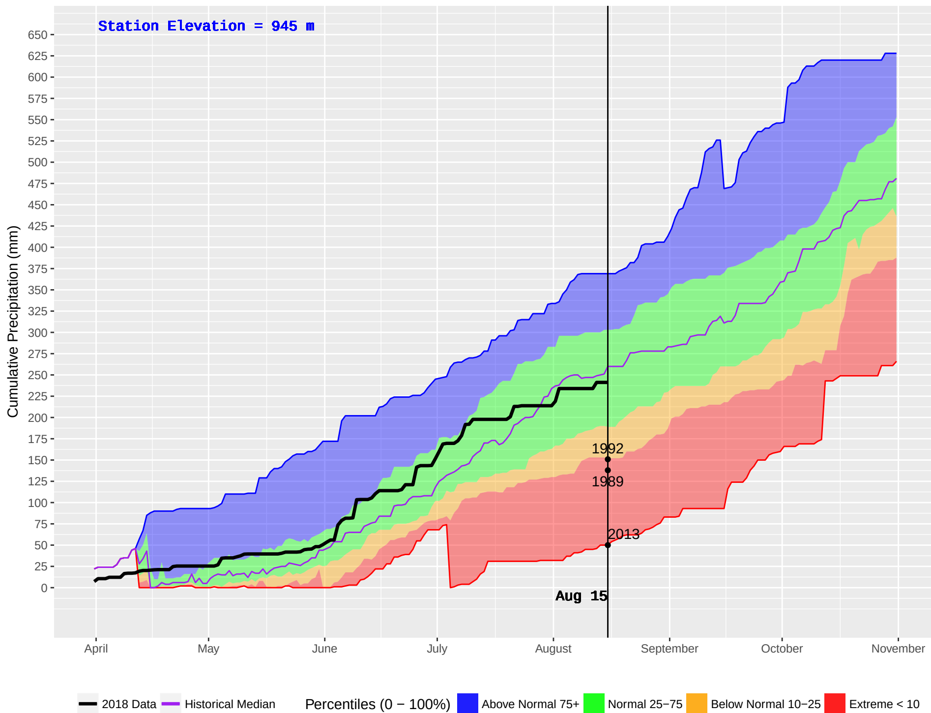
BOWRON HAGGEN (193) : Historical (1986–2016) and Current (2018) Daily Cumulative Precipitation
